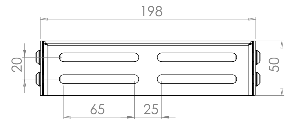
Mount bracket hole pattern
